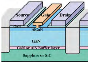
AlGaIn/GaN HEMT
