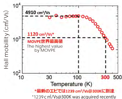
図2. N型低濃度エピのホール移動度 Fig.2 Hall mobility in our n-type low-doping epi-layer
